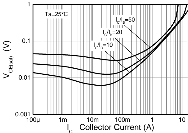
Figure 10. V_{CE(sat)} v I_C
