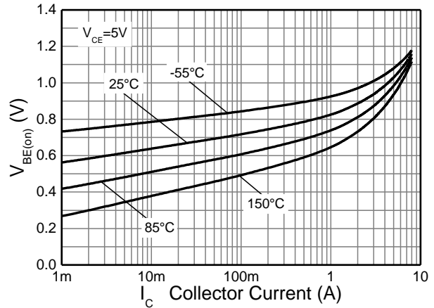
Figure 11. V_{BE(on)} v I_C
