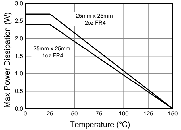
Figure 2. Derating Curve
