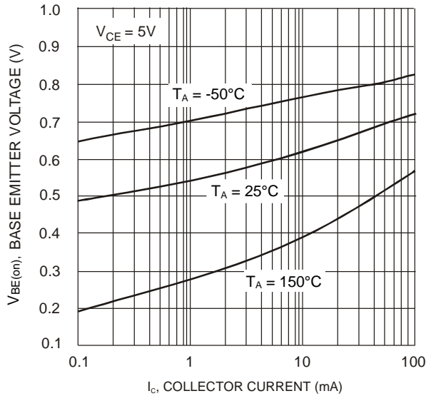
Figure 7. Base Emitter Voltage vs Collector Current
