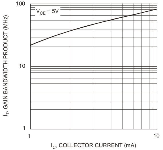
Figure 8. Gain Bandwidth Product vs Collector Current
