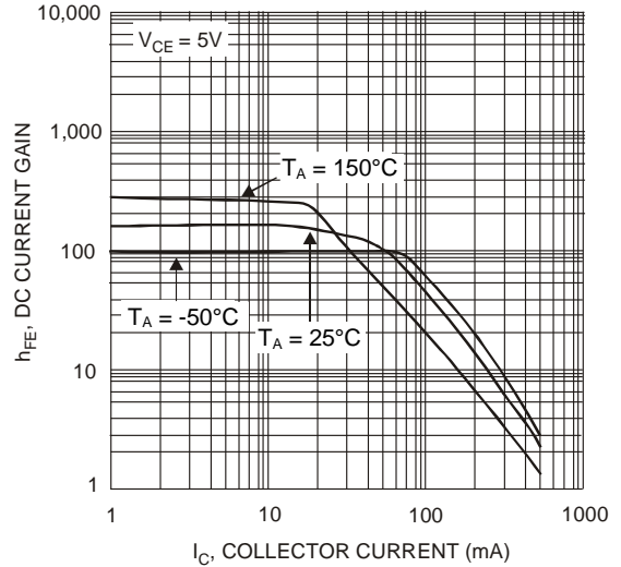
Figure 6. DC Current Gain vs Collector Current
