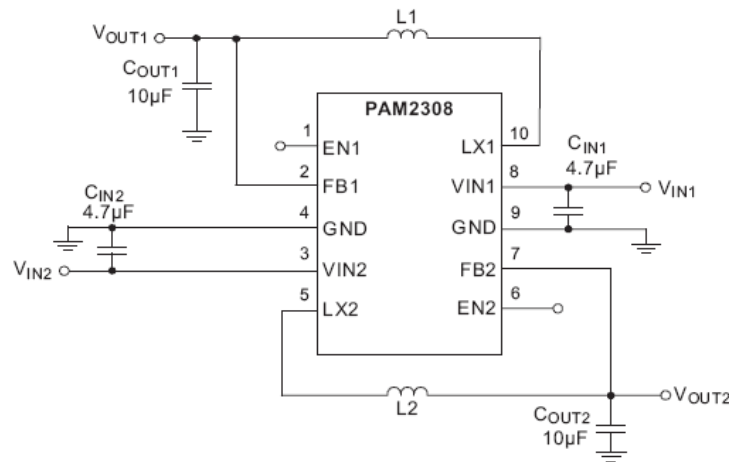
V_{OUTx} = 1.2V, 1.5V, 1.8V, 2.5V, 2.8V or 3.3V Figure 2. Fixed Voltage Regulator
