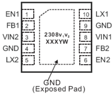
TOP VIEW WDFN-10L 3x3
