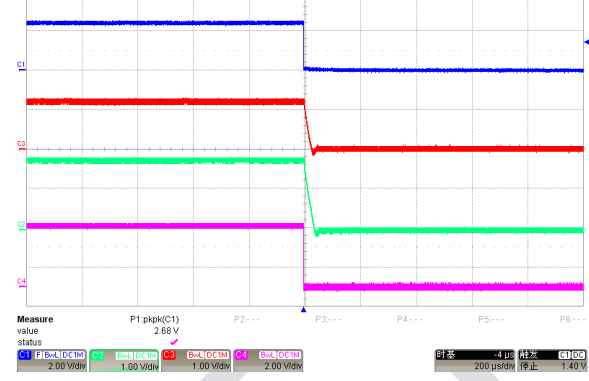
(CH1=Enable; CH2=Vout2; CH3=Vout1; CH4=PG)
