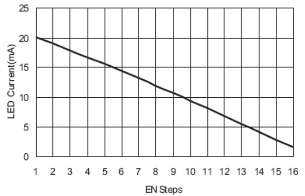
LED Current VS EN Steps
