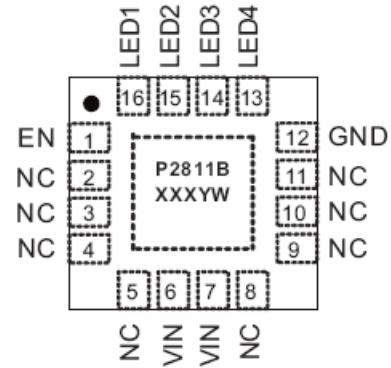
QFN3x3-16L
