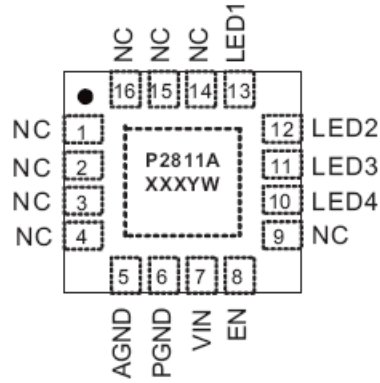
QFN3x3-16L
