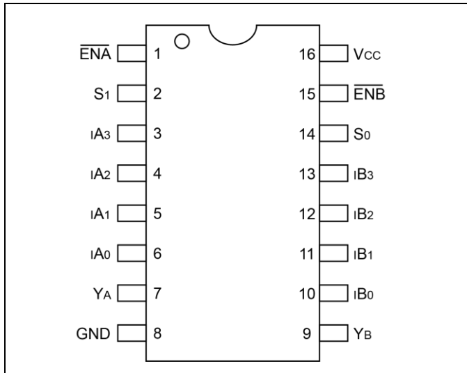
TSSOP/QSOP Package
