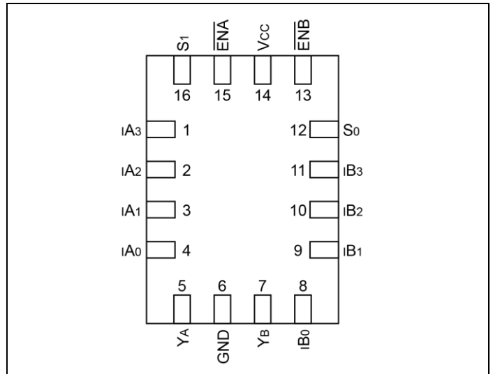
UQFN Package
