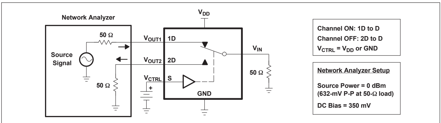
Figure 4. Crosstalk (X TALK )
