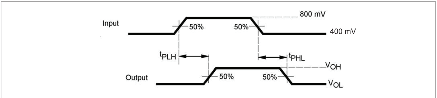
Figure 6. Propagation Delay
