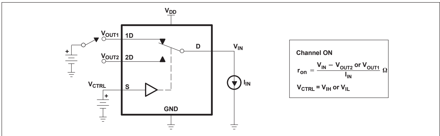
Figure 8. ON-State Resistance ( r_{on} )
