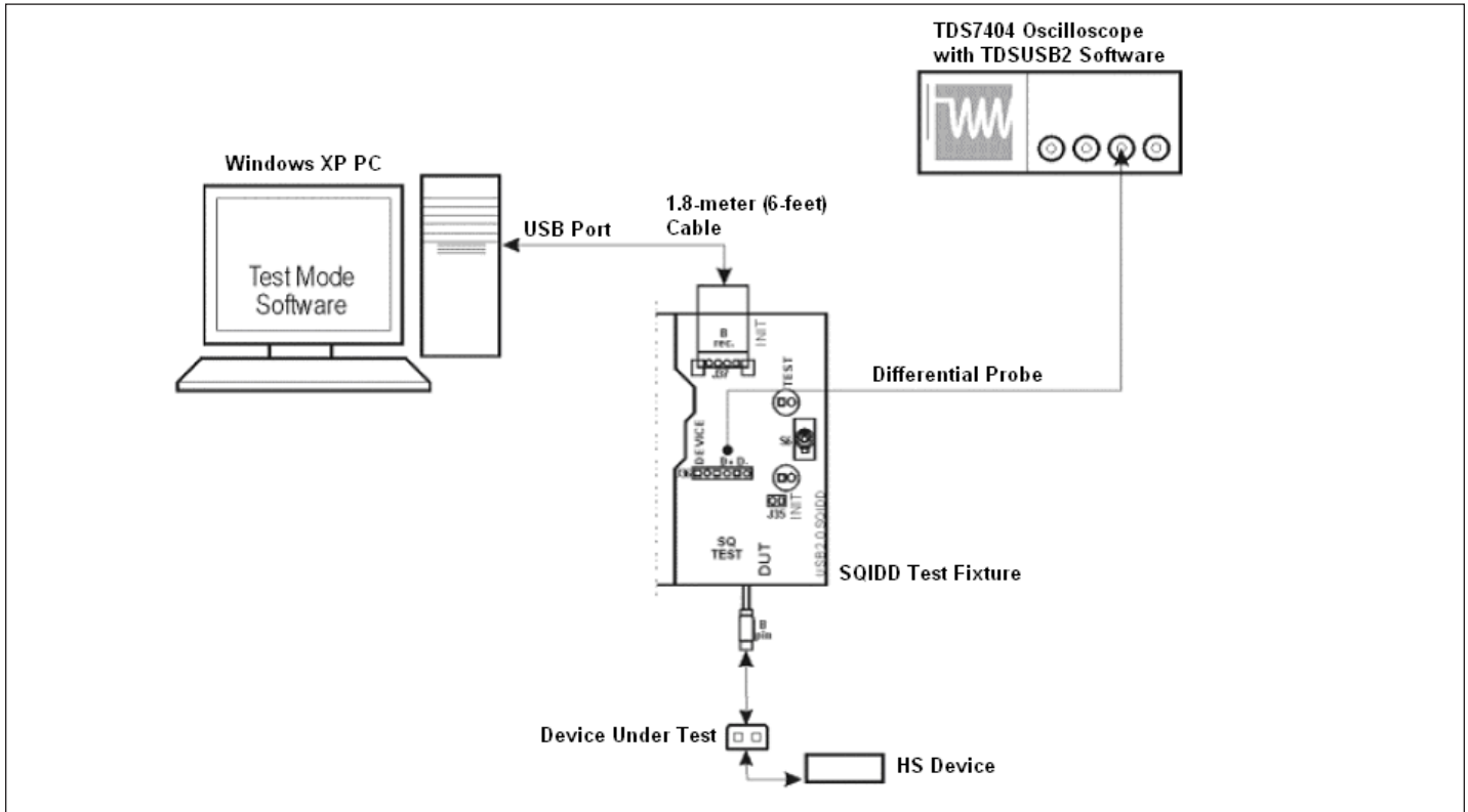
Figure 1. HS Eye Test Setup
