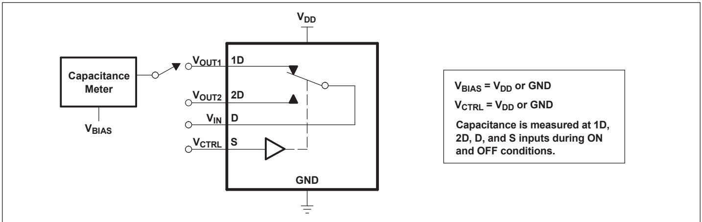
Figure 10. Capacitance
