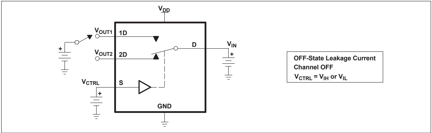
Figure 9. OFF-State Leakage Current
