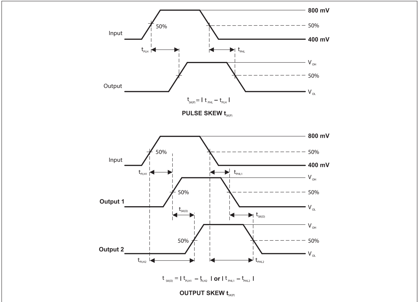
Figure 7. Skew Test
