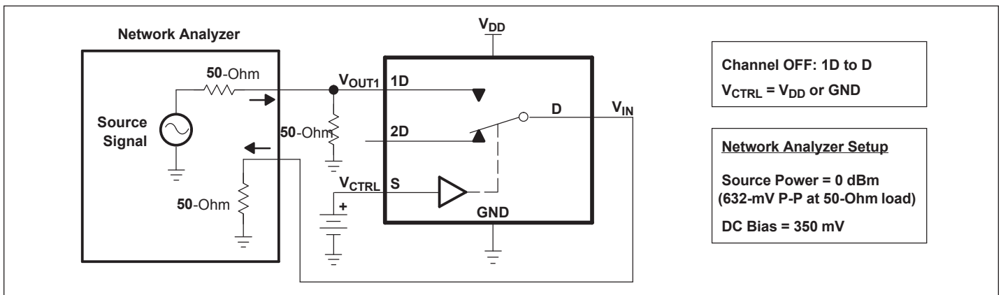
Figure 3. OFF Isolation (O ISO )
