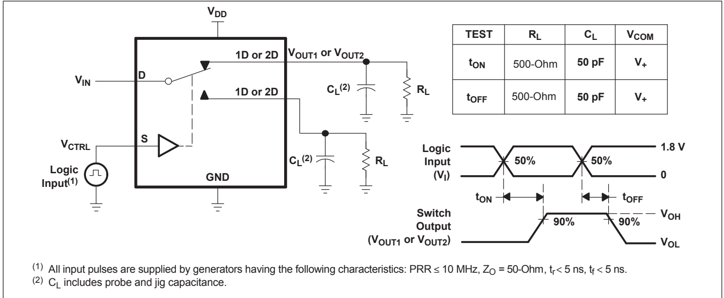
Figure 2. Turn-On (t ON ) and Turn-Off Time (t OFF )
