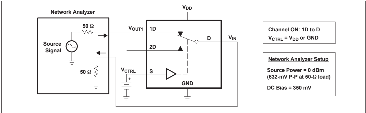
Figure 5. Bandwidth (BW)
