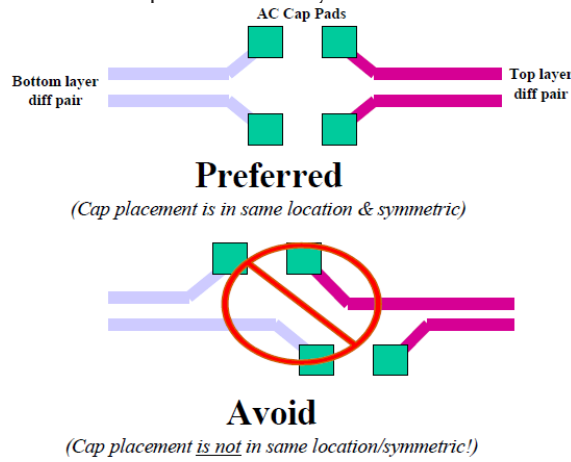
Figure 7-15 Layout Guidance of Series Component
