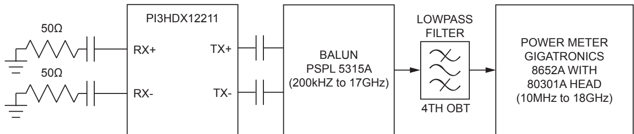
Figure 6-4 Noise Test Configuration
