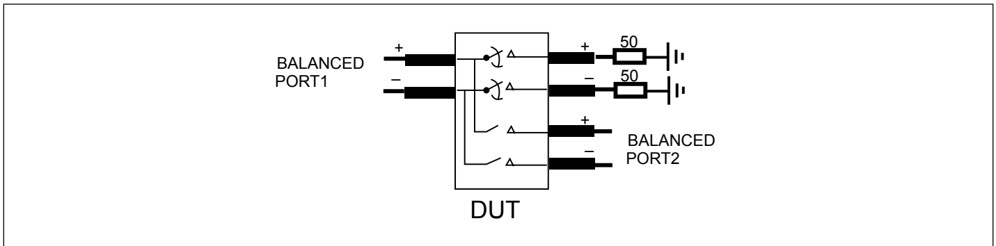
Fig 2. Off-isolation Setup
