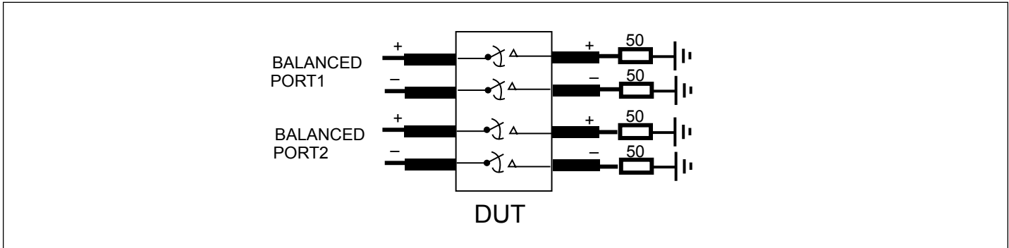
Fig 1. Crosstalk Setup
