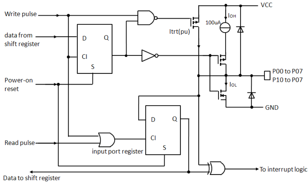
Figure 3. Simplified schematic diagram of P00 to P17
