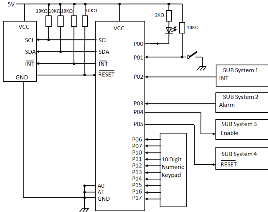
Figure 8. Bidirectional I/O Expander Application
