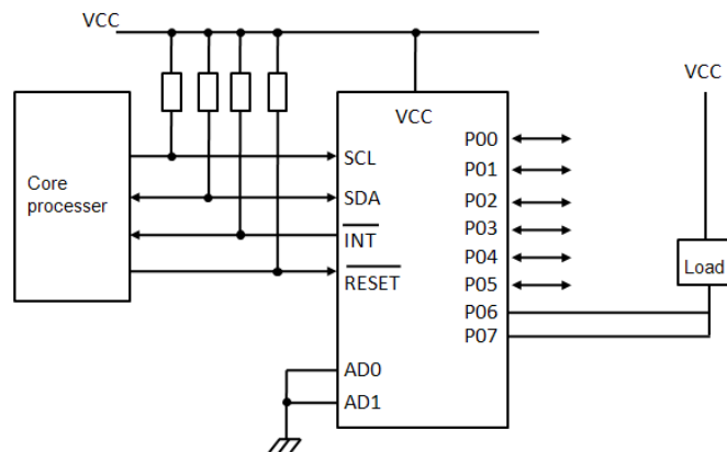
Figure 9. High Current-drive Load Application
