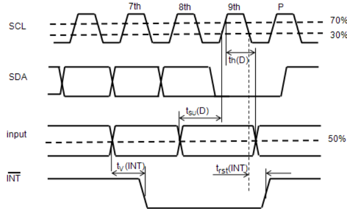
Figure 1. Timing Parameters for INT Signal
