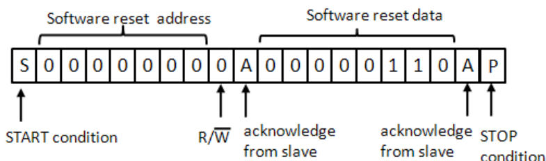
Figure 2. Software Reset Sequence
