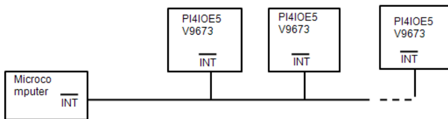
Figure 7. Application of Multiple P4IOE5V9673s with Interrupt
