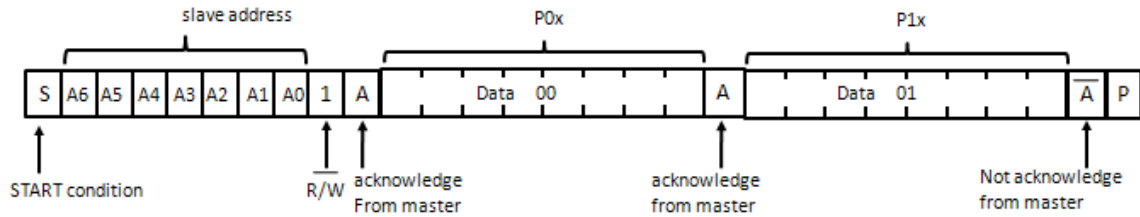
Figure 6. Read Input Port Register
