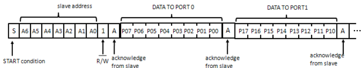
Figure 5. Write Mode
