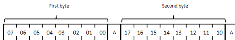
Figure 4. Correlation between Bits and Ports
