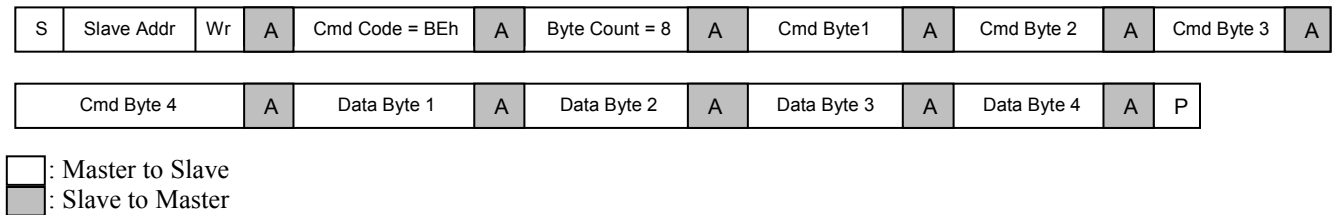
Figure 7-2 SMBus Block Write Command Format, to Write to a PI7C9X2G1616PR Register without PEC
