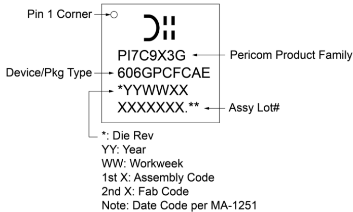
Figure 14-2 Part Marking
