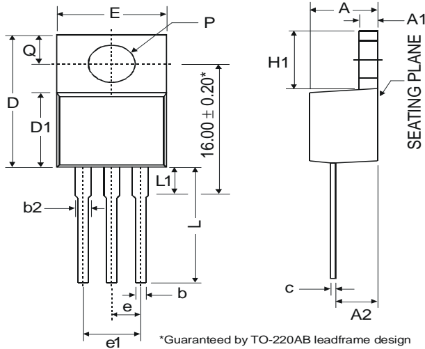
TO-220AB
