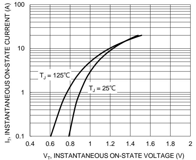
Figure 6. On-State Characteristics
