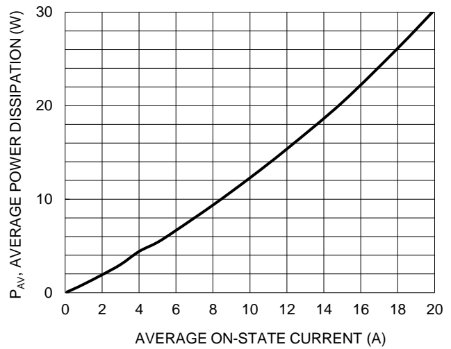
Figure 4. On-State Power Dissipation
