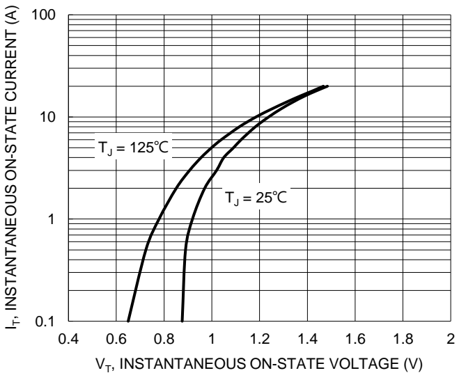
Figure 12. On-State Characteristics
