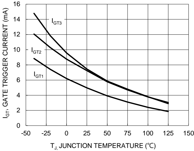
Figure 1. Typical Gate Trigger Current vs. Junction Temperature
