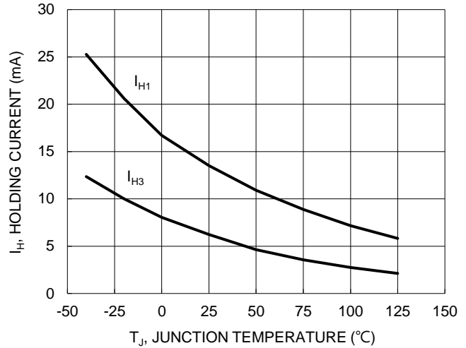
Figure 2. Typical Holding Current vs. Junction Temperature
