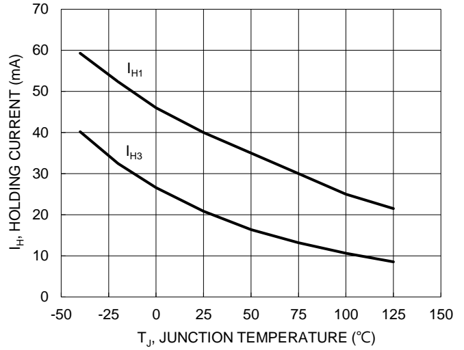
Figure 8. Typical Holding Current vs. Junction Temperature
