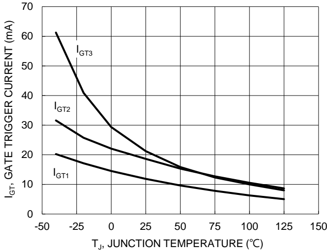
Figure 7. Typical Gate Trigger Current vs. Junction Temperature
