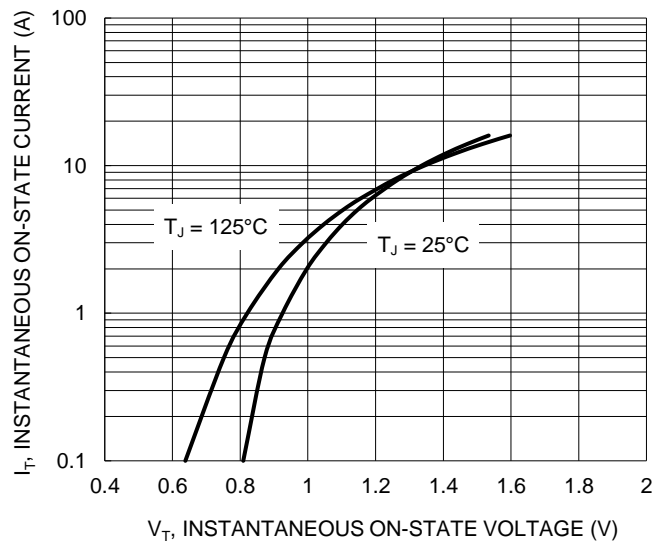
Figure 6. On-State Characteristics
