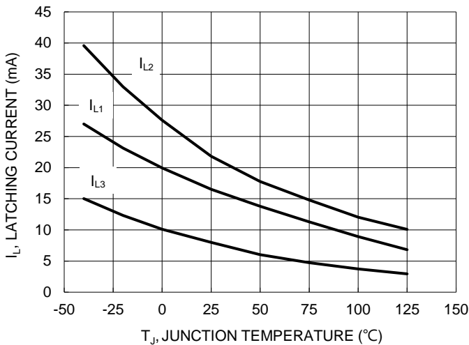
Figure 3. Typical Latching Current vs. Junction Temperature
