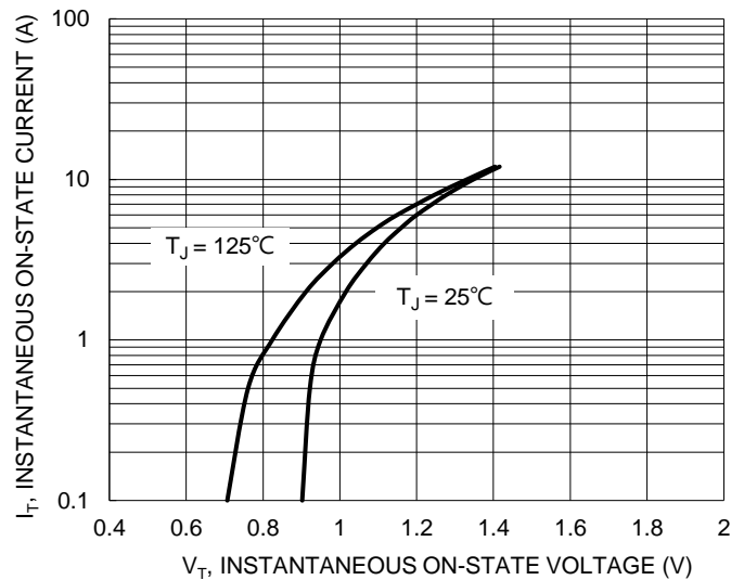
Figure 12. On-State Characteristics
