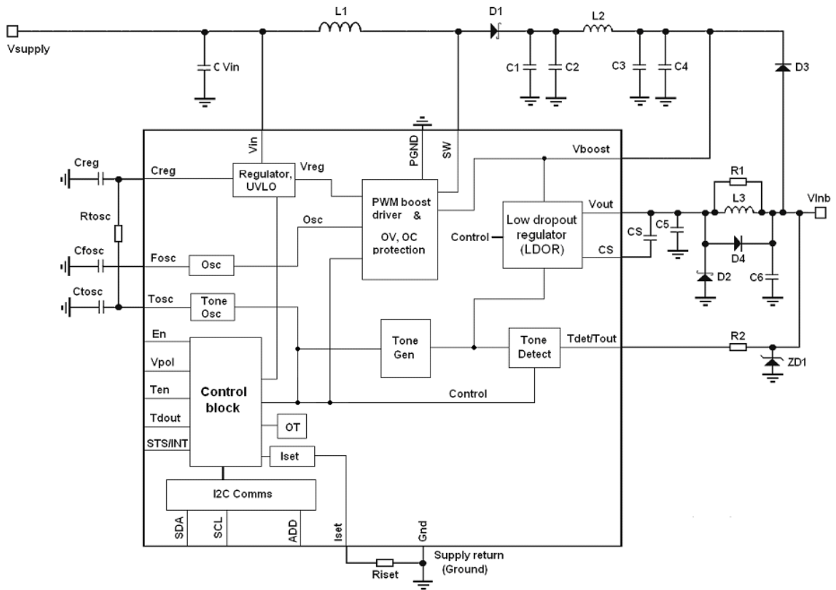
Figure. 1 ZLPM8011 Functional Diagram and Application Circuit for a DiSEqC 2 System
