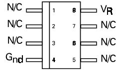
S08 Package Suffix – N8
