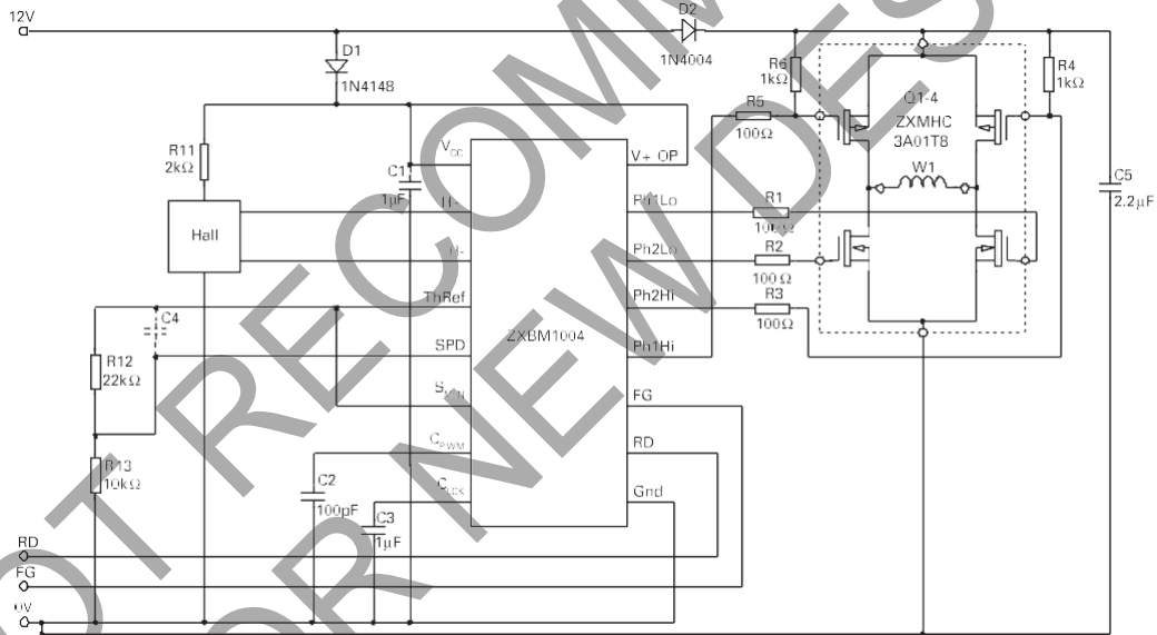
Figure 4. Typical Circuit for Constant Speed Operation
