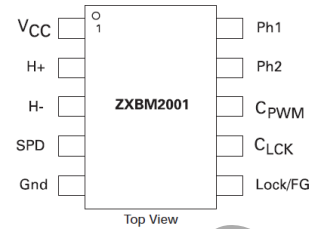
MSOP-10
