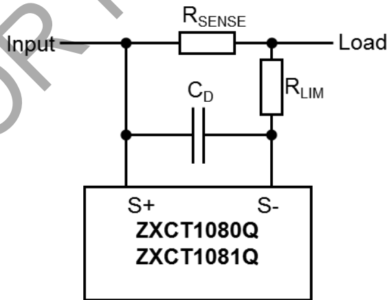
Fig. 21 Protection/Error Sources for ZXCT1080Q/81Q
