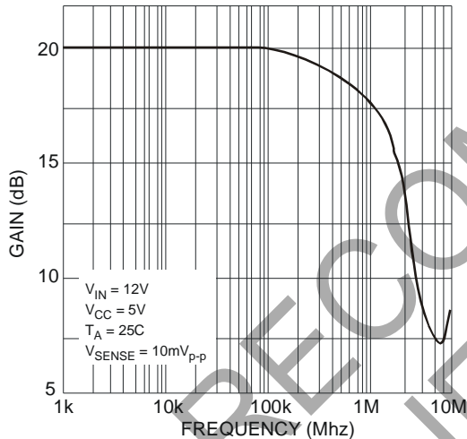
Fig. 14 Small Signal Bandwidth
