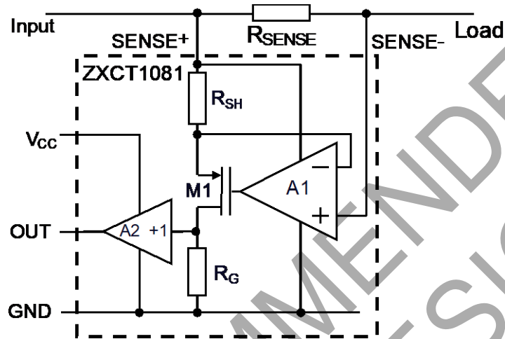
Figure 1. Typical Configuration of ZXCT1081
