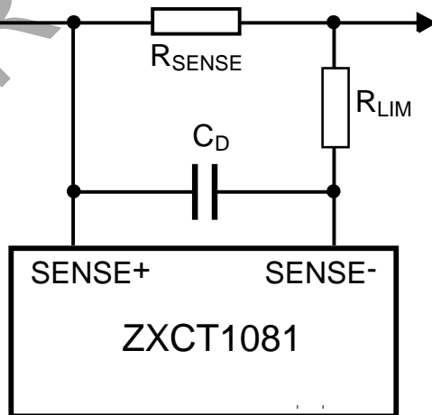
Figure 2. Protection/Error Sources for ZXCT1081
