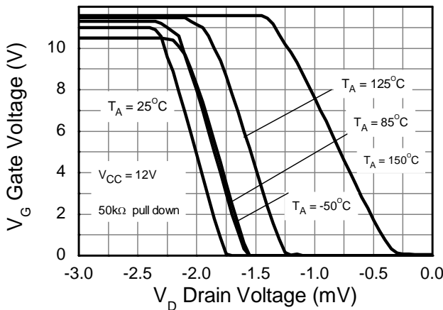
Transfer Characteristic
