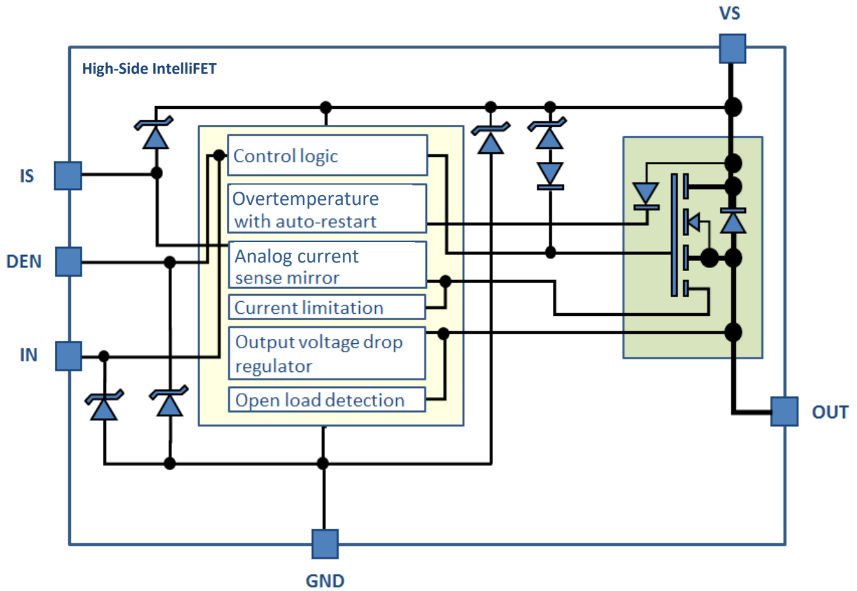
Figure 2. Functional Block Diagram of ZXMS81200SP
