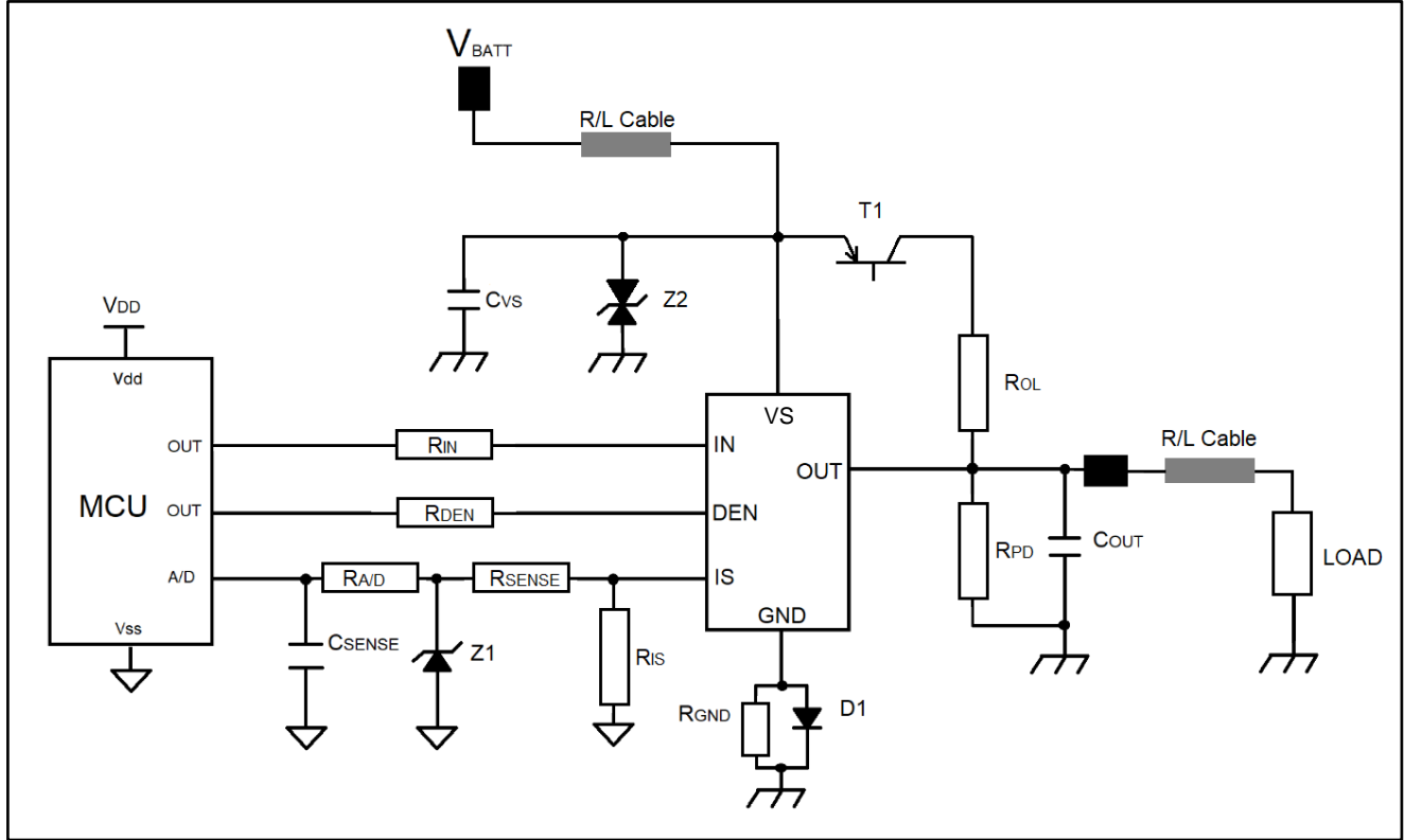
Figure 37. Application Diagram
