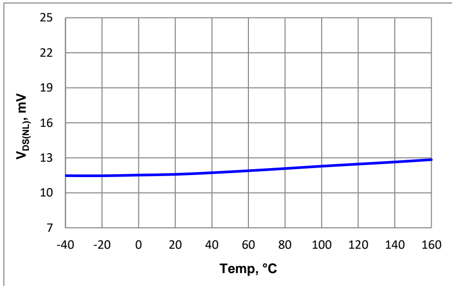
Figure 4. Output Voltage Drop Regulation, I_{OUT} = 50\text{mA}
