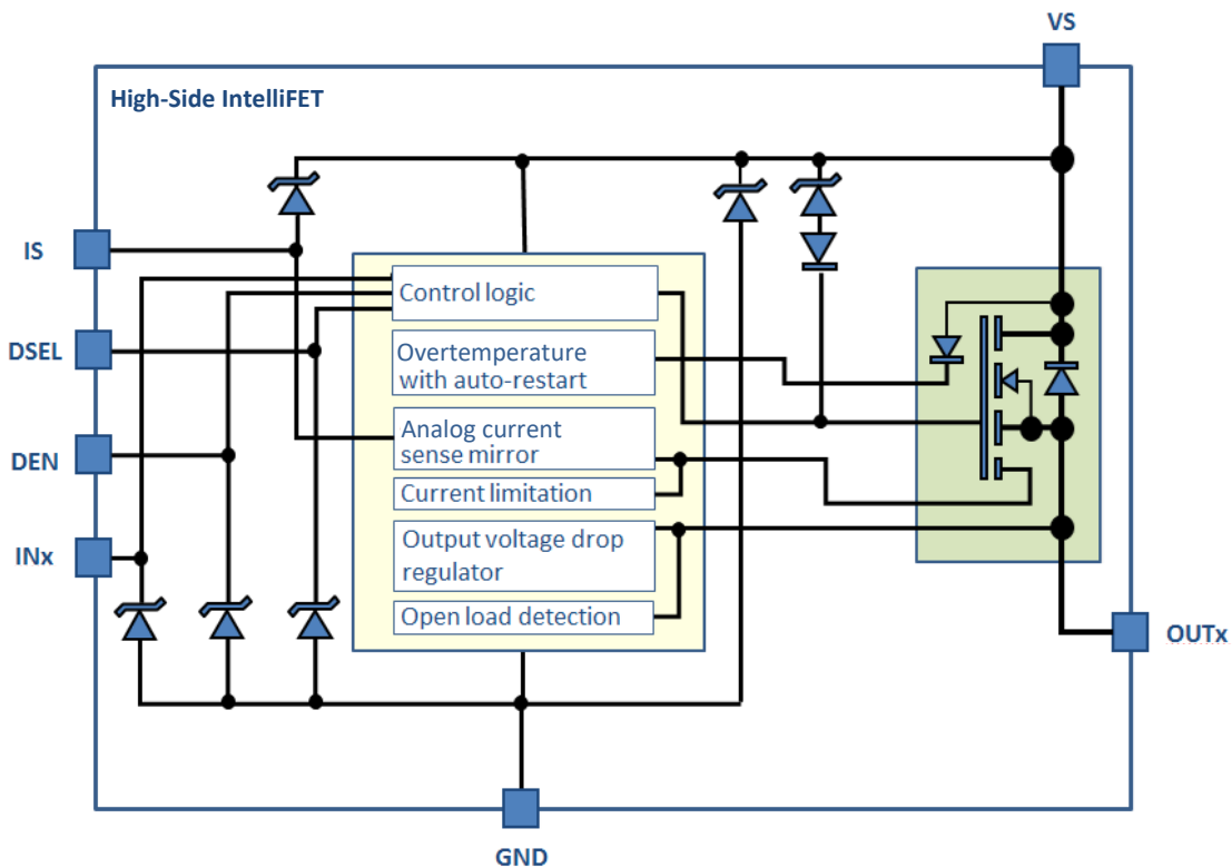
Figure 2. Functional Block Diagram of ZXMS82090S14P
